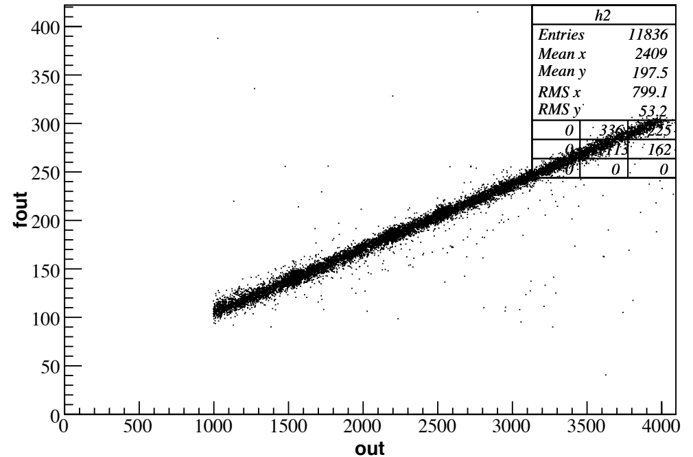
1st cycle sdd4 no vertex cut (Kaon timing)
