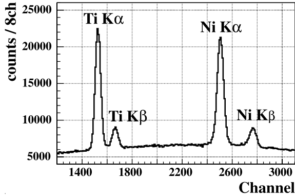
Figure 1: A typical characteristic X-ray spectrum with calibration self trigger.
