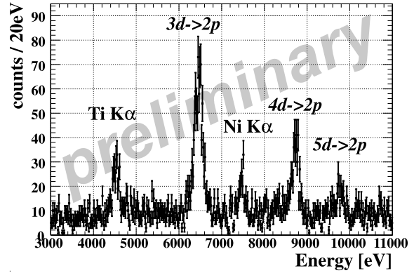
Figure 2: Preliminary kaonic helium atom X-ray energy spectrum for half of all E570 statistics.
